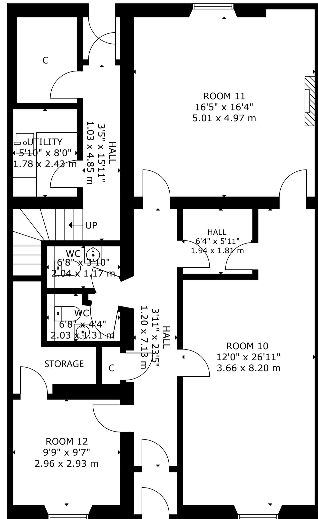
BASEMENT
